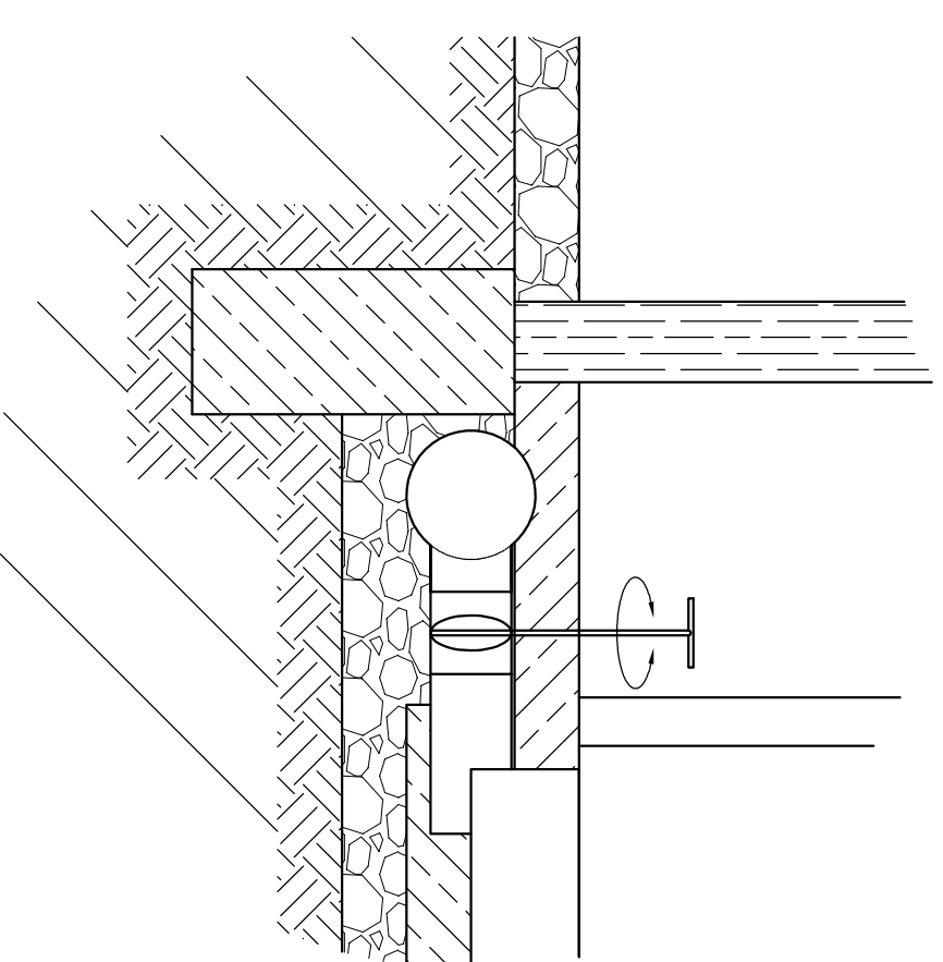
Detail view 1 Scale 1 : 25
